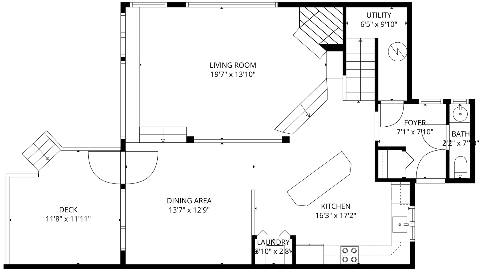
Main Level
